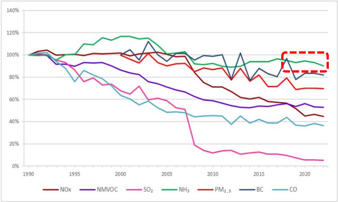
Figure 0.8.1 Relative variation of air pollutants emissions (100 % in 1990 or 2000 for PM and BC)
